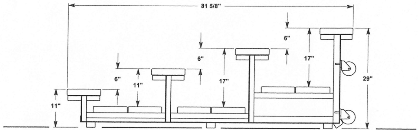
FANSTAND 4 Row w/double footplank Tip N Roll Bleacher
