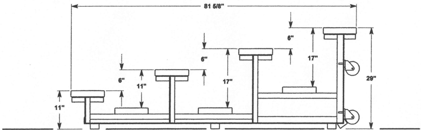
FANSTAND 4 Row w/single footplank Tip N Roll Bleacher
